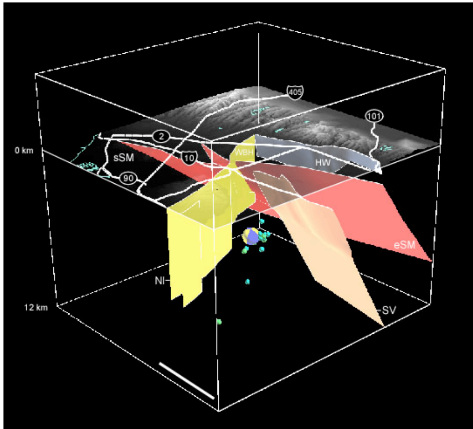
Fig.2: Perspective view of the faults (NI=Newport-Inglewood fault, WBH=West Beverly Hills Lineament, SV=San Vicente fault, sSM=Santa Monica (Southern Strand) fault, eSM=eastern segment of the St. Monica fault which coincides in parts with the North Salt Lake fault, HW=Hollywood fault) in the vicinity of the earthquake. The focal mechanism of the main shock is represented as a large sphere (600 m radius), and the aftershocks as small spheres (blue and green). Topography is shown as a grey, transparent and shaded DEM.
